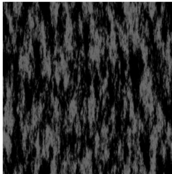
OLD_06_S
