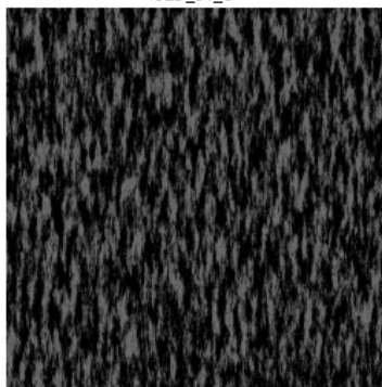
OLD_05_S
