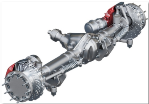
Front_Axle
