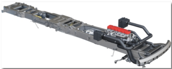
Defence_Truck_10
