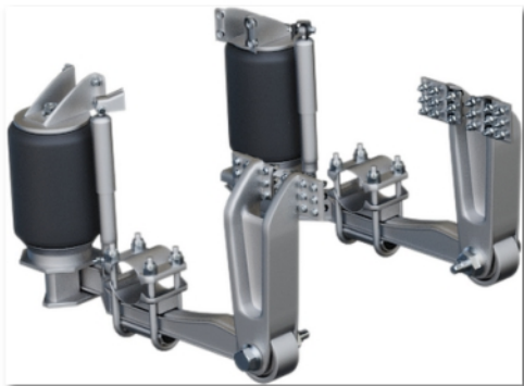
Rear_Suspension
