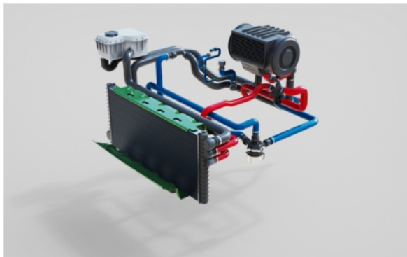
Cooling_Control_System
