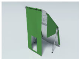
practice_net_10
